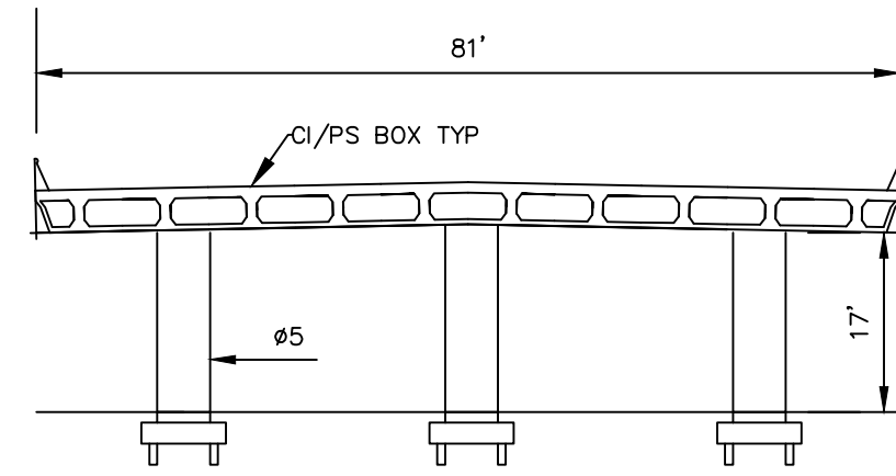
TYPICAL SECTION 1"=20'
