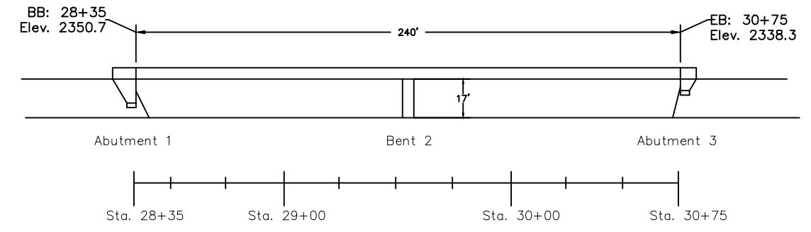
ELEVATION 1"=60'
