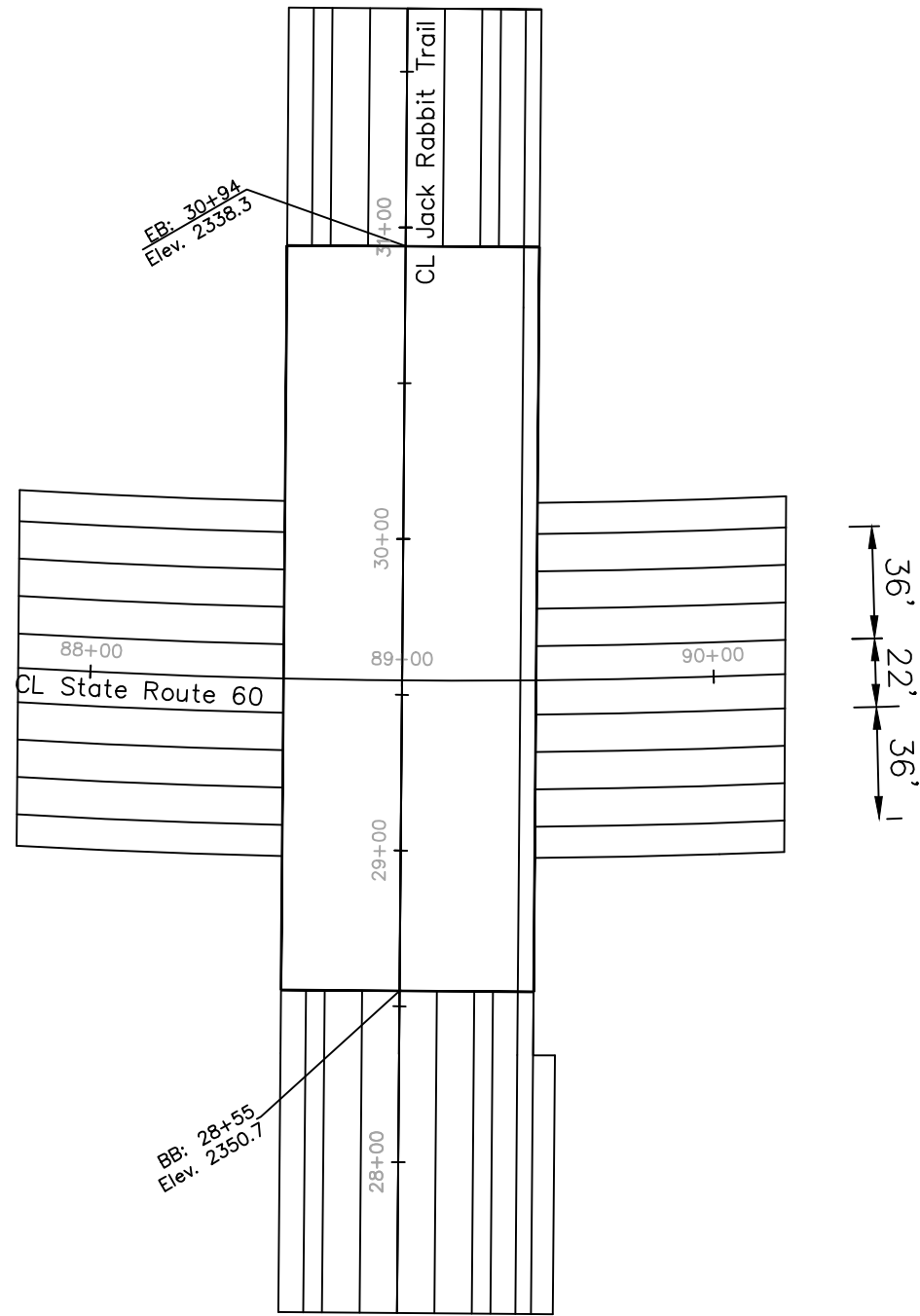
PLAN 1"=70'
